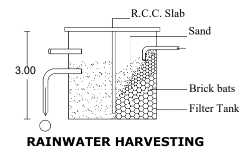
RAINWATER HARVESTING
