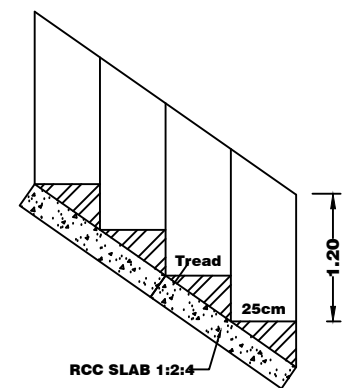
STAIR DETAILS
