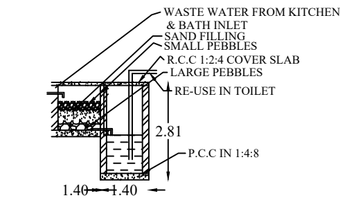
RECYCLING OF WASTE WATER KITCHEN & BATHROOM
