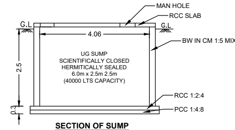
SECTION OF SUMP
