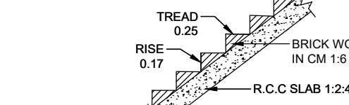
STAIRCASE DETAILS
