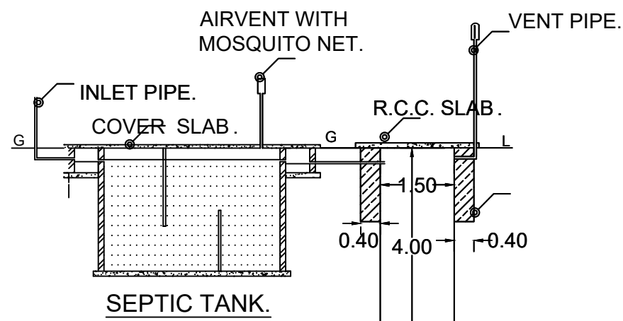
SOAK PIT SECTION.
