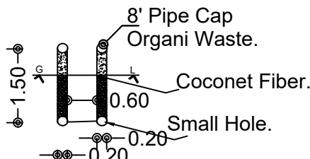
COMPOST PIT
