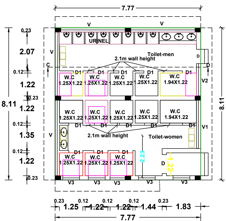
TOILET PLAN (BLOCK-2)
