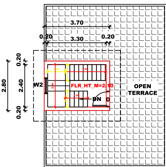
HEAD ROOM PLAN
