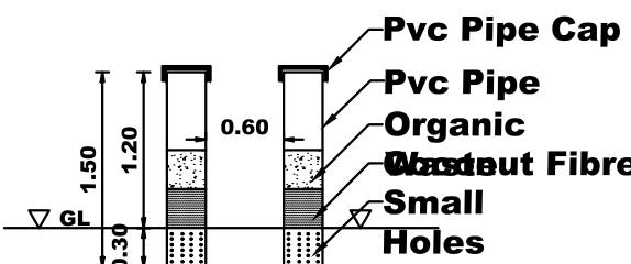
PIPE COMPOST PIT
