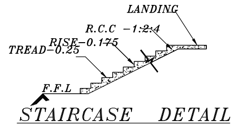
STAIRCASE DETAIL
