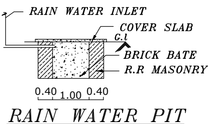
RAIN WATER PIT
