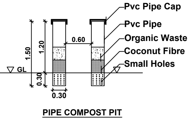
PIPE COMPOST PIT
