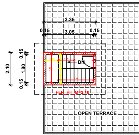
HEAD ROOM PLAN
