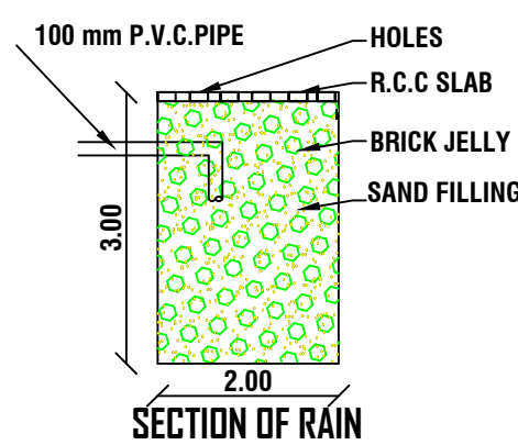
SECTION OF RAIN
