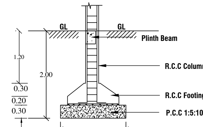
SECTION OF COLUMN
