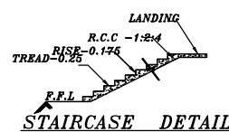
STAIRCASE DETAIL
