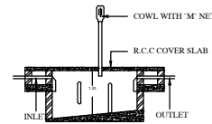
SEPTIC TANK DETAILS
