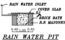
RAIN WATER PIT
