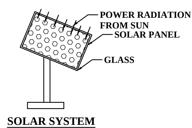
SOLAR SYSTEM
