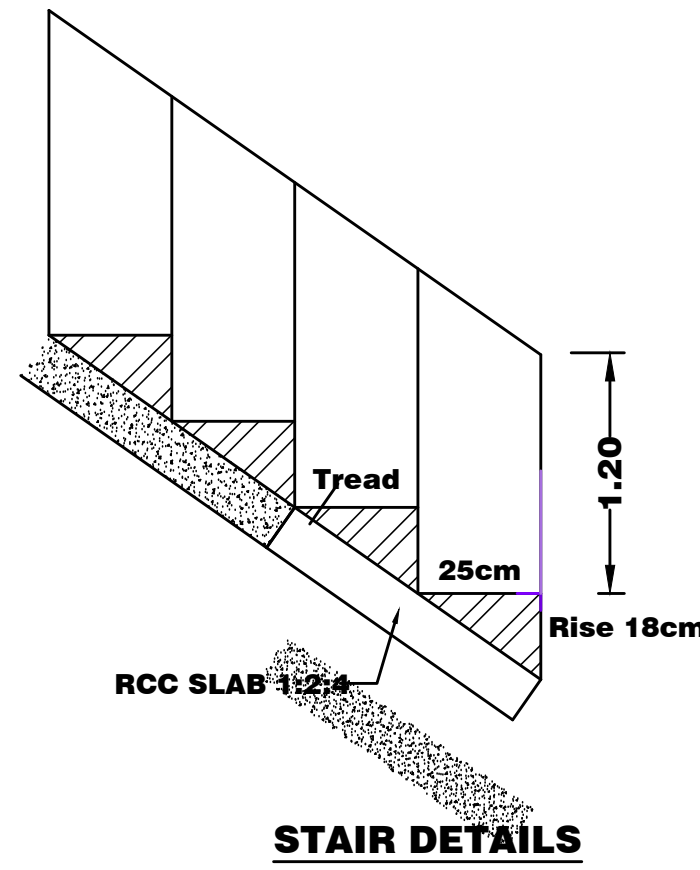
STAIR DETAILS
