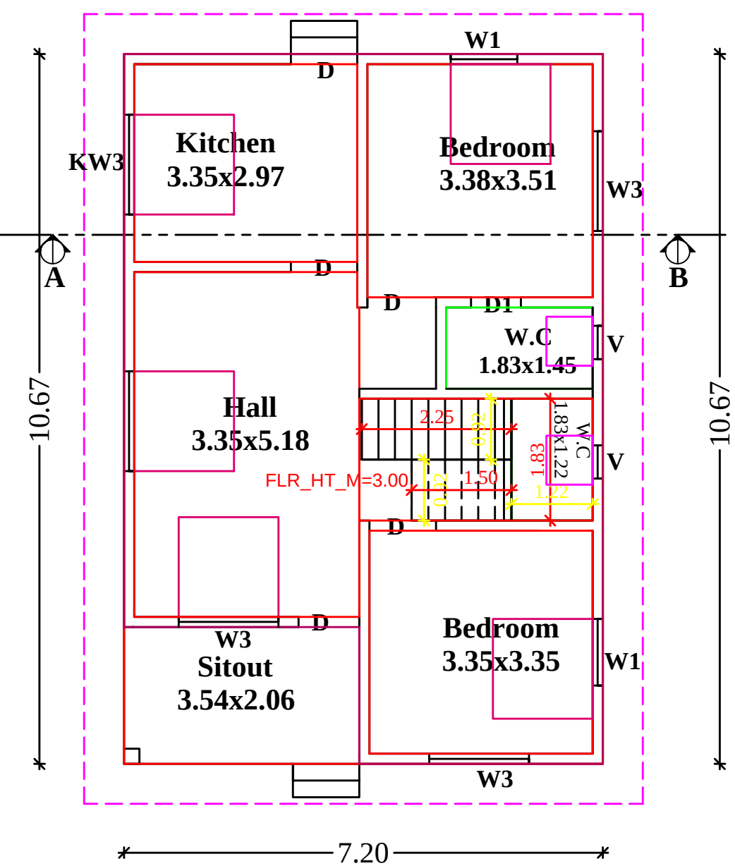
PLAN
