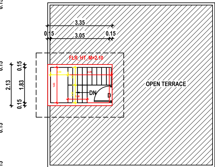
HEAD ROOM PLAN
