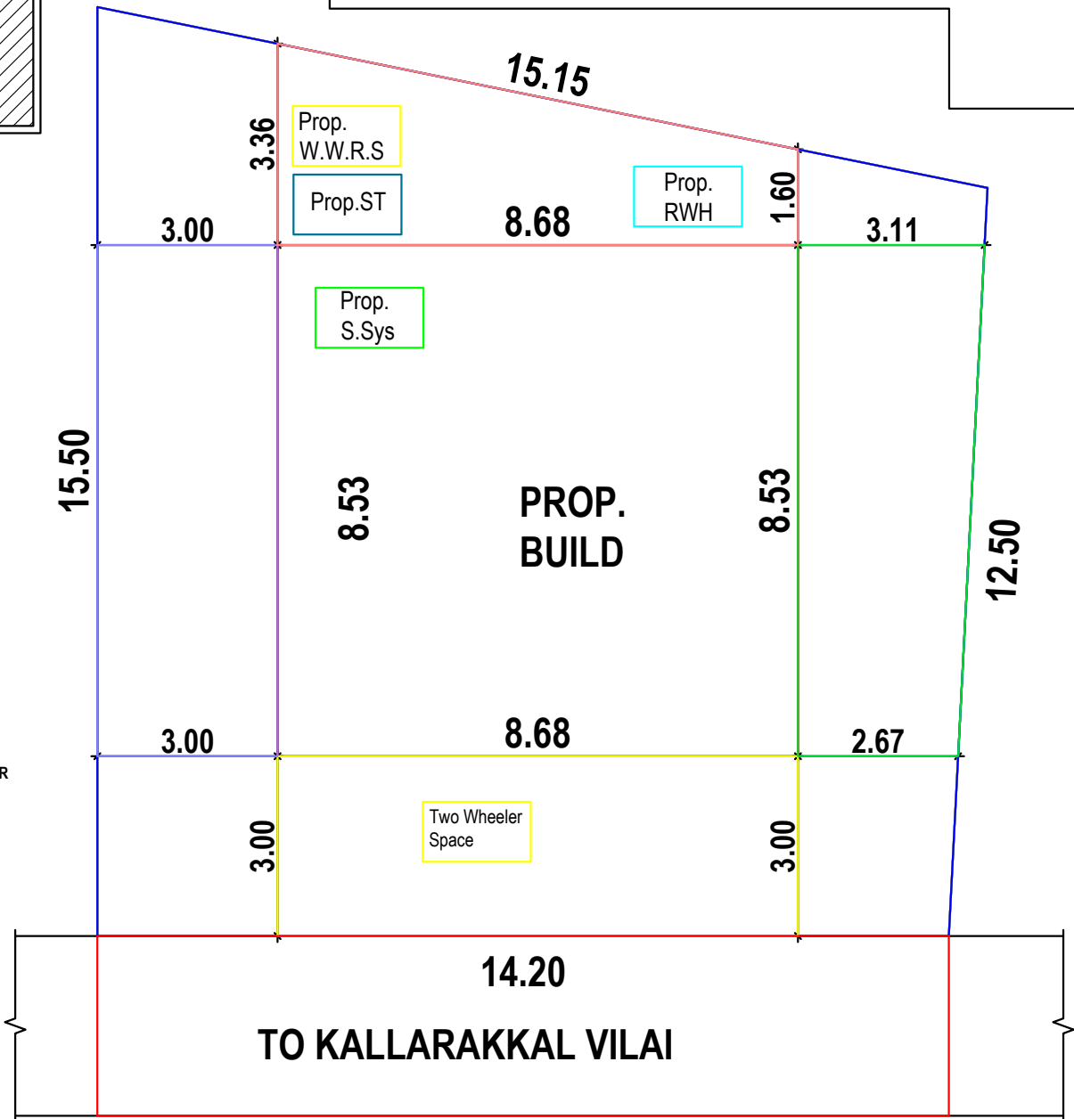
SITE PLAN
