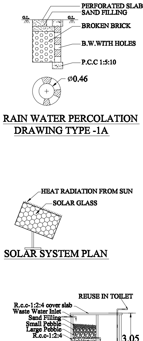
RAIN WATER PERCOLATION DRAWING TYPE -1A
