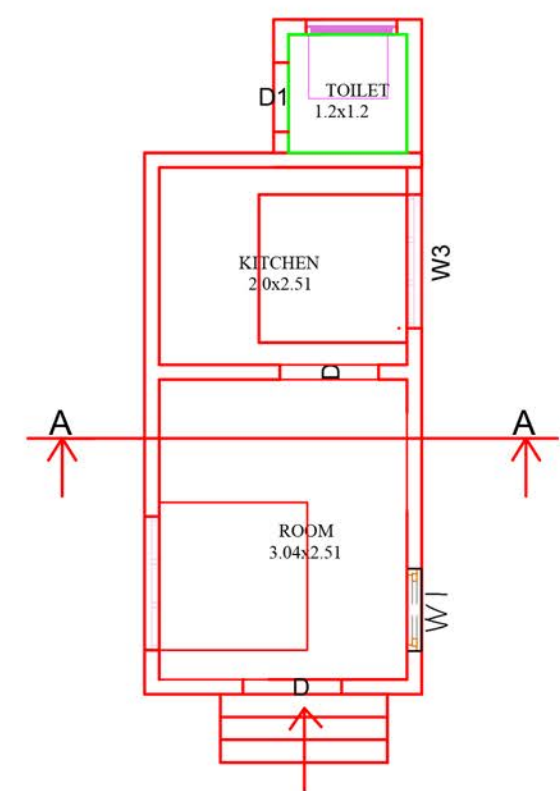
GROUND FLOOR PLAN (facing north )
