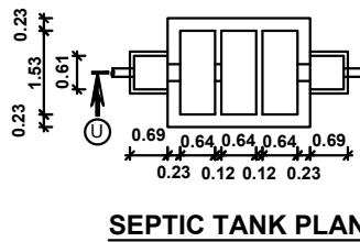
SEPTIC TANK PLAN
