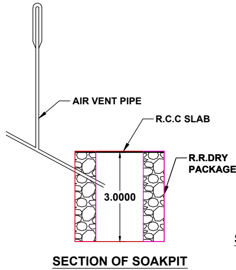
SECTION OF SOAKPIT
