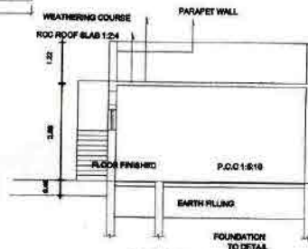
SECTION "A-B"
