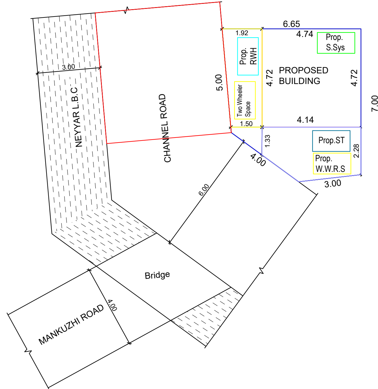
SITE PLAN
