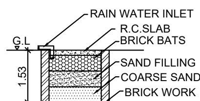
RAIN WATER
