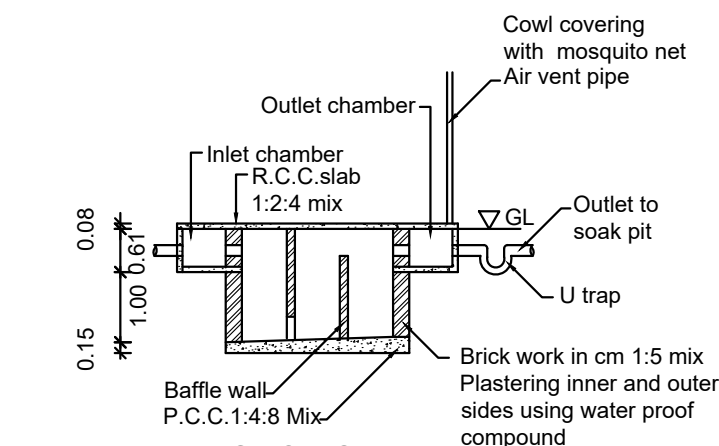
SECTION UV
