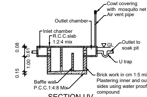
SECTION UV
