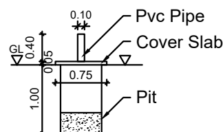
SOLID WASTE COMPOST PIT
