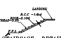
STAIRCASE DETAIL
