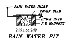
RAIN WATER PIT
