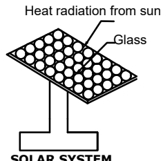
SOLAR SYSTEM
