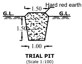
TRIAL PIT
