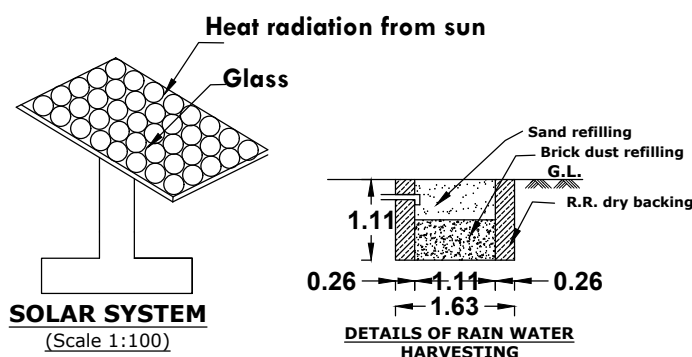
DETAILS OF RAIN WATER HARVESTING
