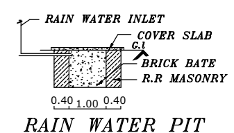
RAIN WATER PIT
