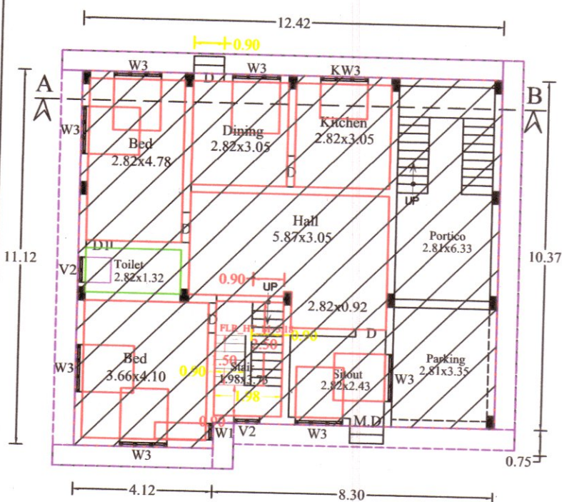
EXISTING GROUND FLOOR PLAN DOOR NO:- 11/10/1
