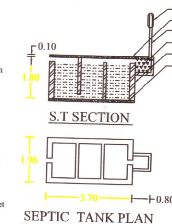
SEPTIC TANK PLAN
