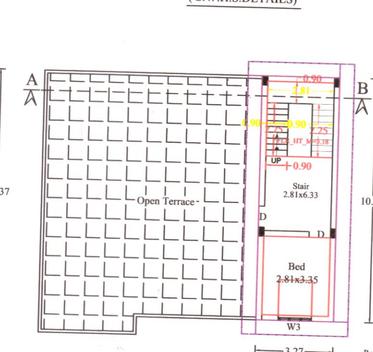
EXTENSION SECOND FLOOR PLAN
