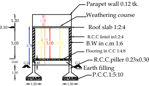
SECTION @ A-B
