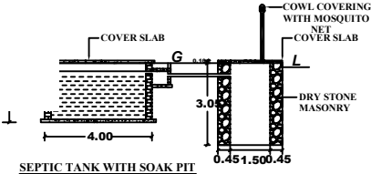
SEPTIC TANK WITH SOAK PIT
