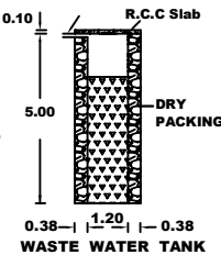
WASTE WATER TANK
