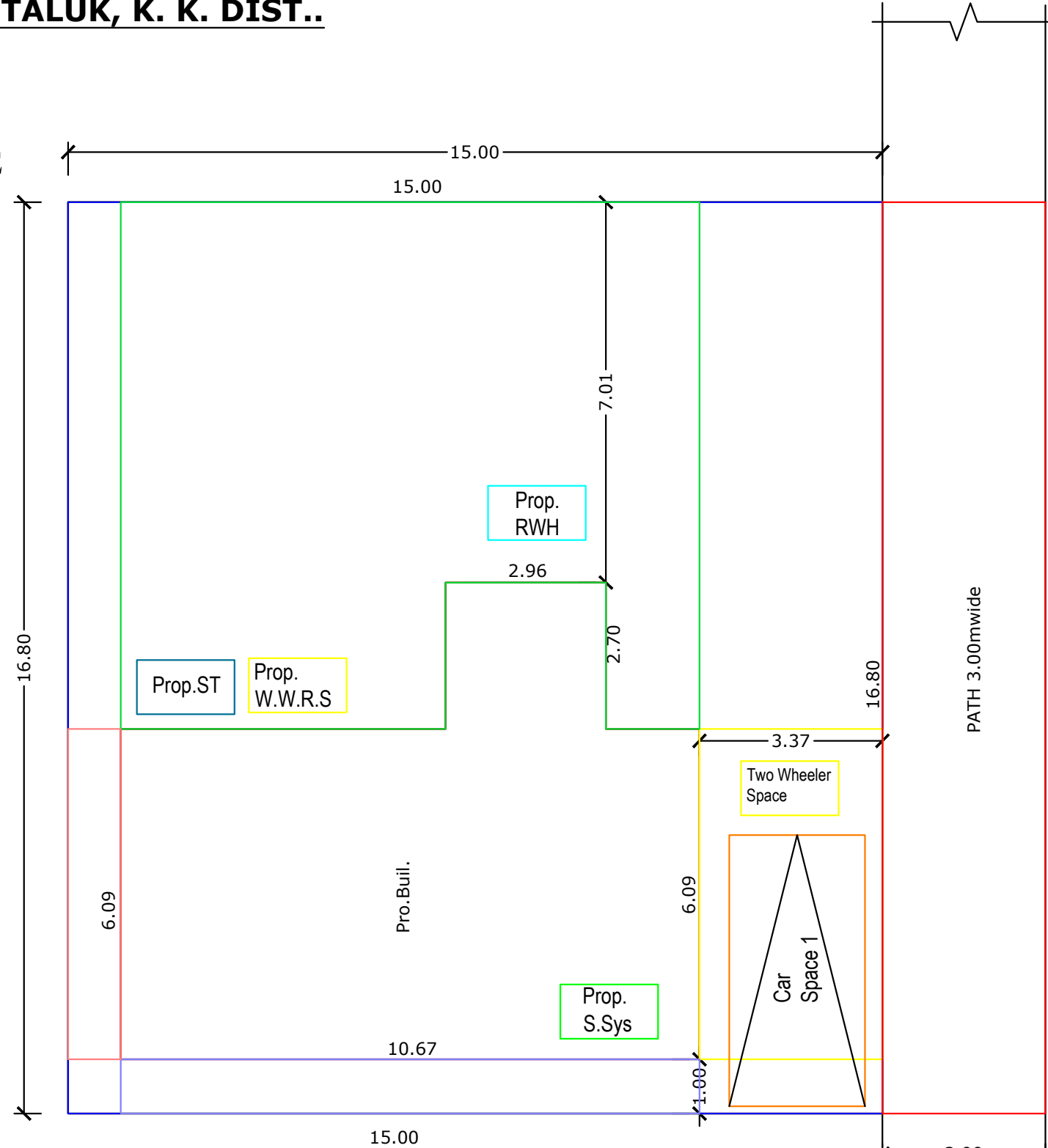
KEY PLAN
