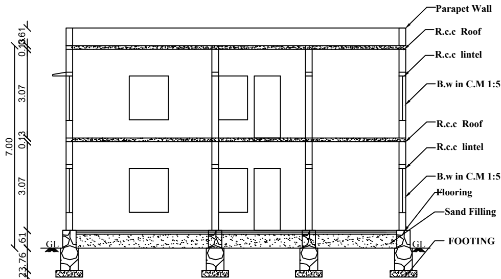
SECTION AB
