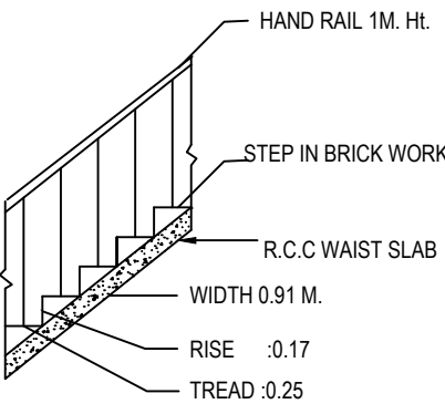
STAIR DETAIL
