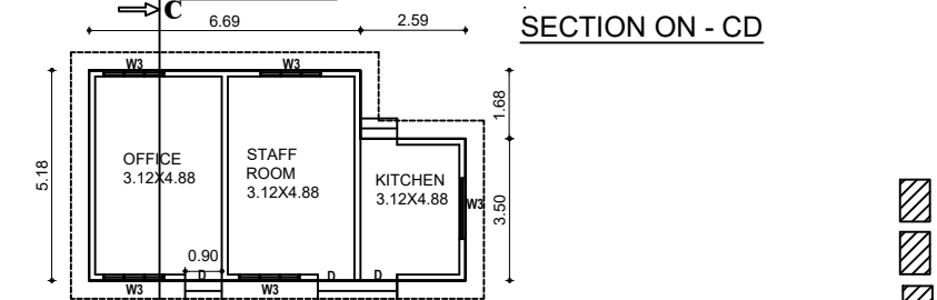
OFFICE, STAFF ROOM KITCHEN - PLAN
