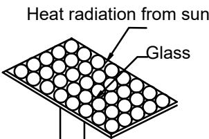
SOLAR SYSTEM (Scale 1:100)
