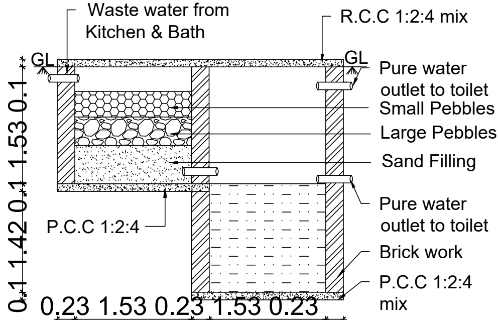
WASTE WATER RECYCLING PIT
