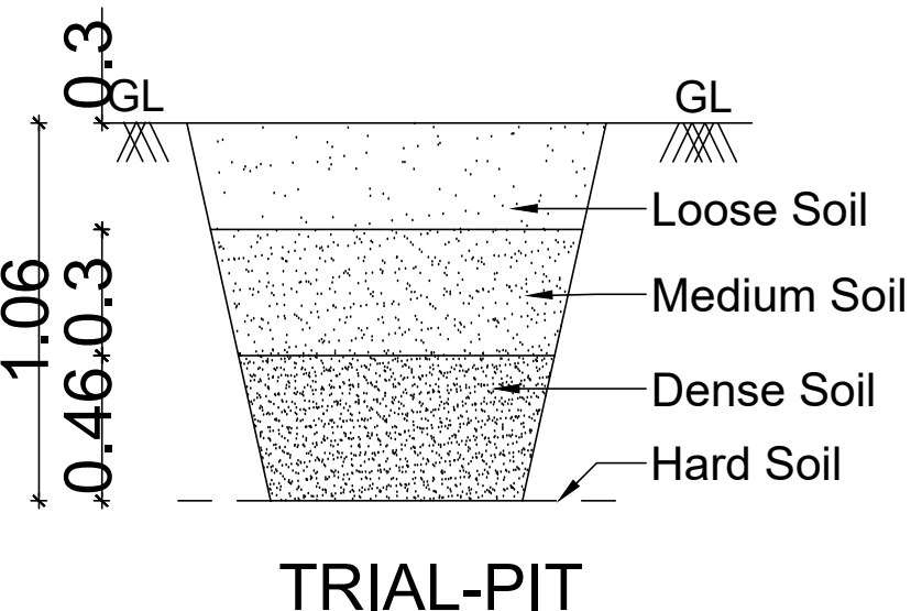
TRIAL-PIT
