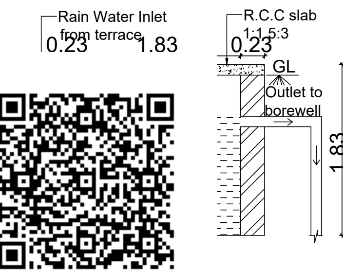
RAIN WATER RECYCLING PIT
