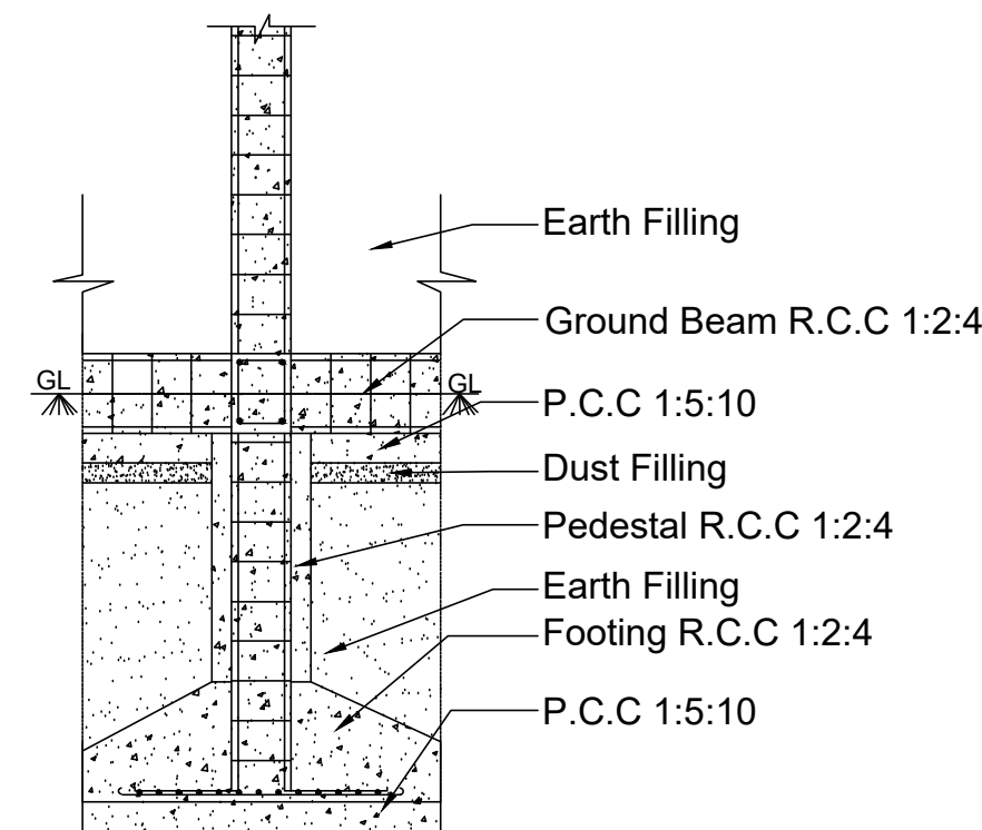
DETAILS OF R.C.C COLUMN
