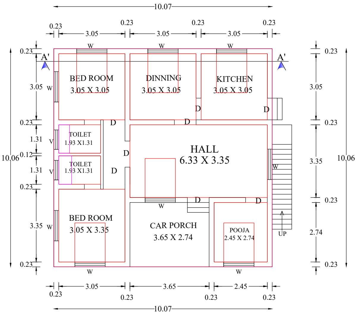
GROUND FLOOR
