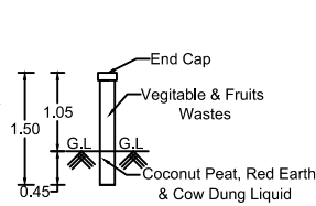
PIPE COMPOSTER
