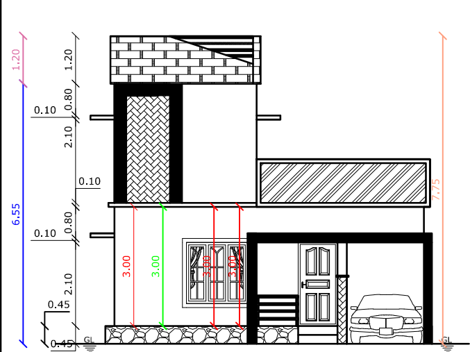
FRONT ELEVATION
