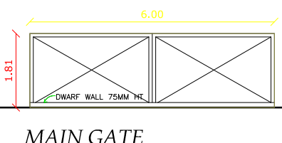
MAIN GATE
