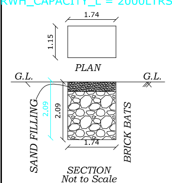
DETAILED PLAN OF RAINWATER PERCOLATION PEBBLE BED
