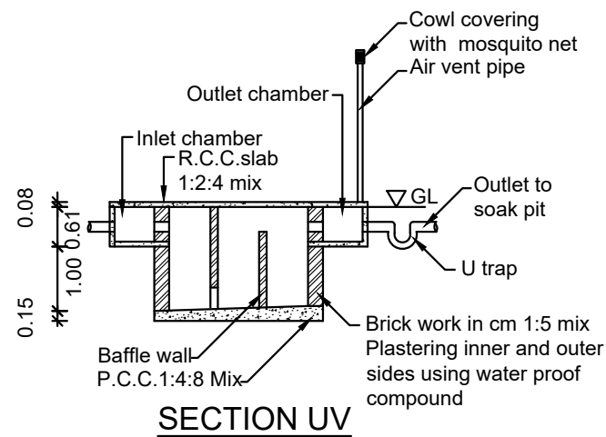
SECTION UV
