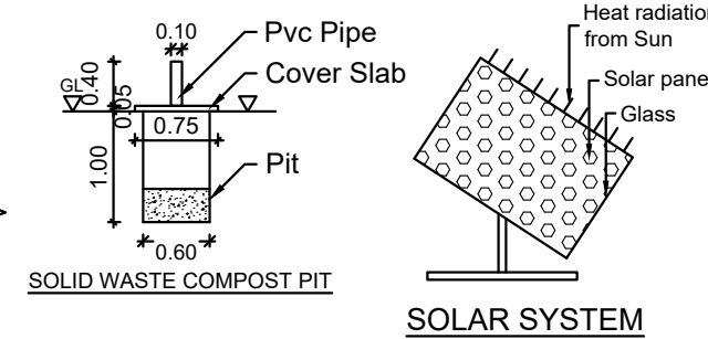
SOLAR SYSTEM
