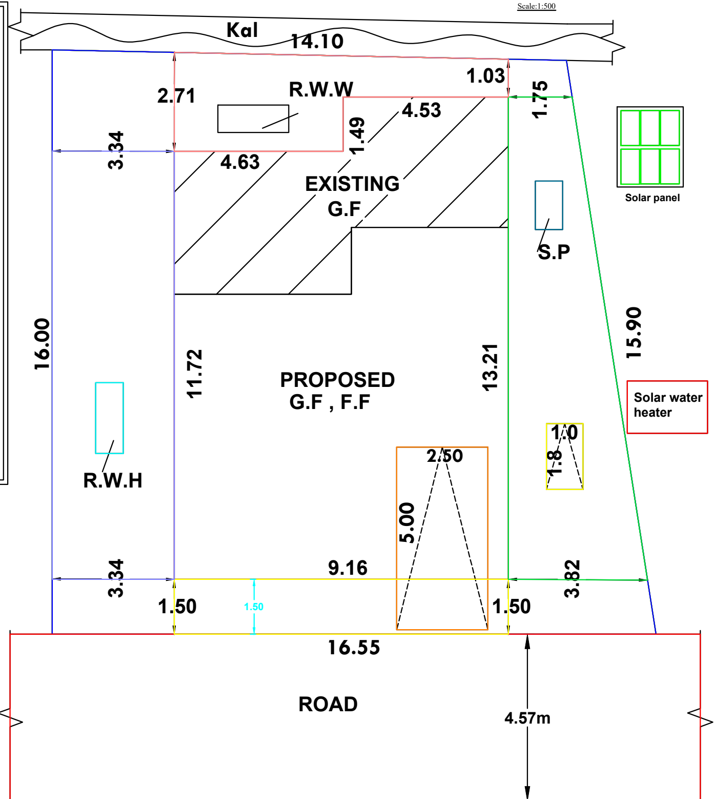
SITE PLAN
