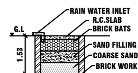
RAIN WATER HARVESTING PIT
