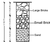
SECTION OF RAIN WATER COLLECTION PITS. (NTS)
