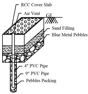
Percolation Bore Pit
