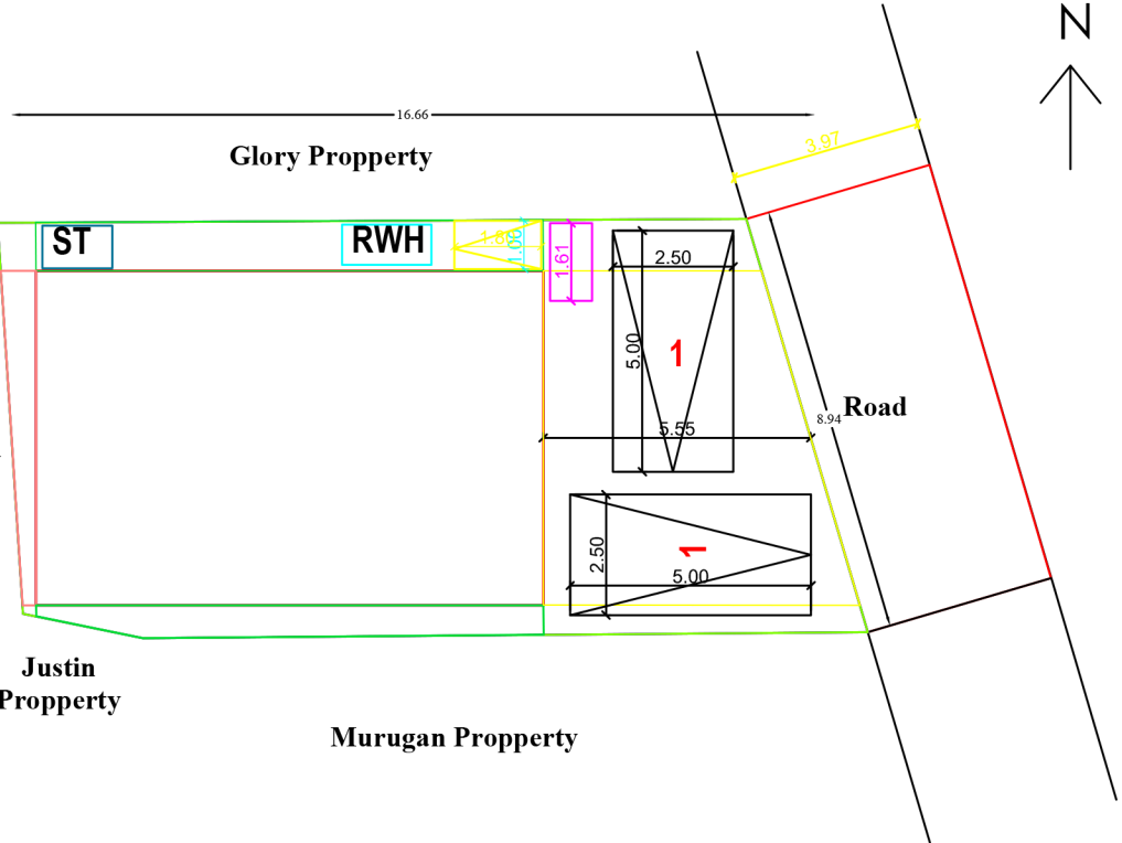
SITE PLAN
