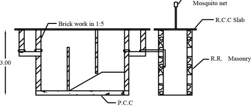
Section of Septic Tank & Soakpit
