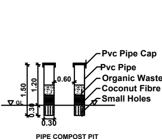
PIPE COMPOST PIT
