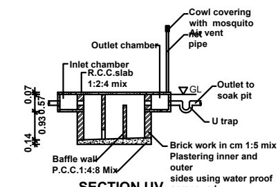
SECTION UV
