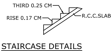
STAIRCASE DETAILS
