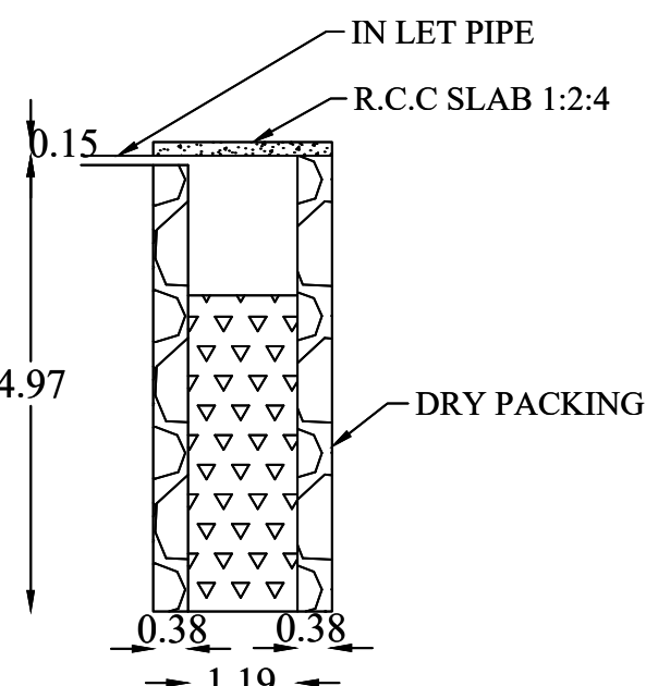
WASTE WATER TANK
