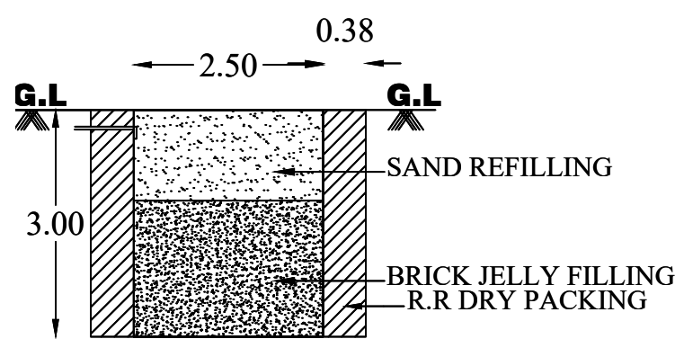
RAINWATER HARVESTING
