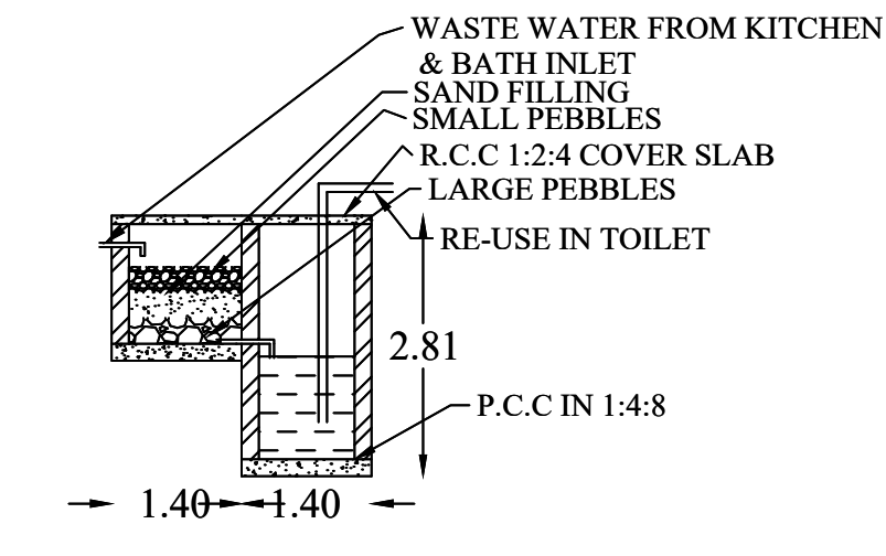
RECYCLING OF WASTE WATER KITCHEN & BATHROOM
