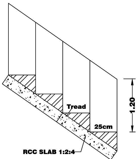
STAIR DETAILS
