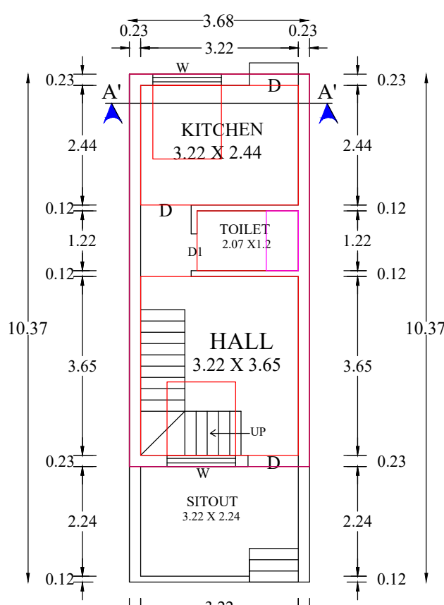
D FLOOR
