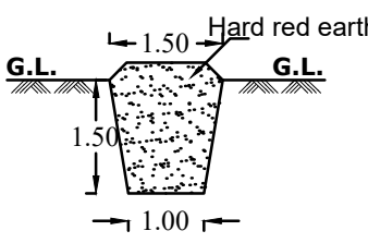
TRIAL PIT (Scale 1:100)
