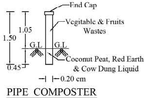
PIPE COMPOSTER
