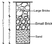
SECTION OF RAIN WATER COLLECTION PITS. (NTS)
