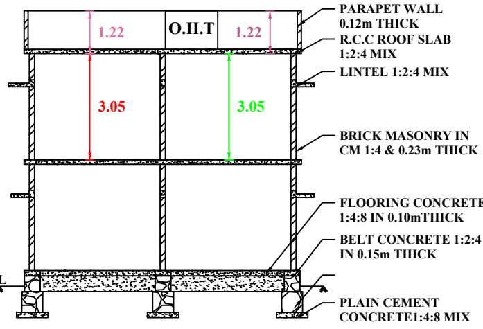
SECTION 'X-Y'
