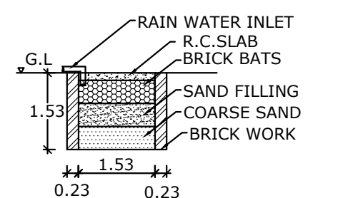
RAINWATERHARVESTING
