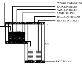
RECYCLING OF WASTE WATER FROM BATH
